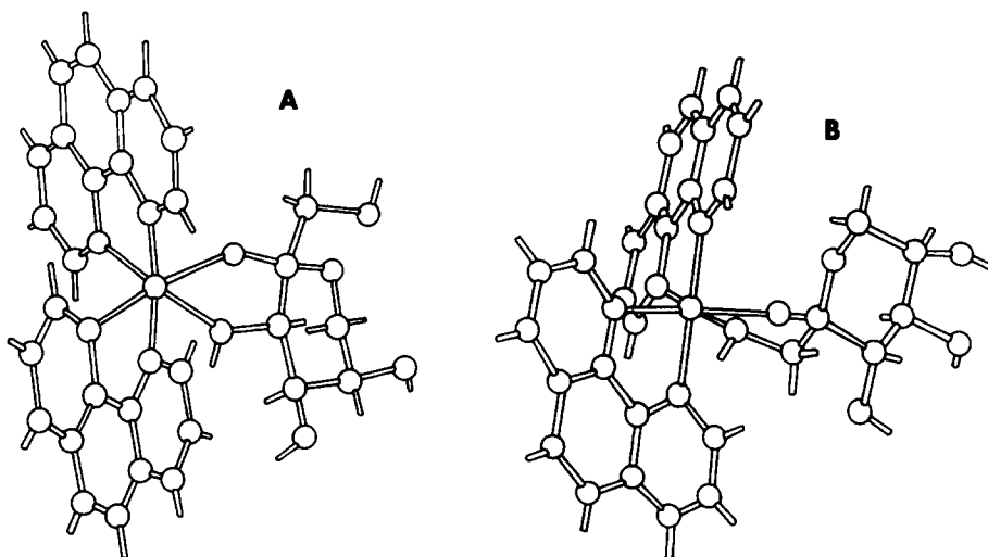
Fig. 4. Simulated structures of the \Lambda -complexes of \text{Co(III)(phen)}_2 with D-fructopyranose with coordination at (A) oxygens at positions 2 and 3 and (B) oxygens at positions 1 and 2. Hydrogens are indicated by sticks.
