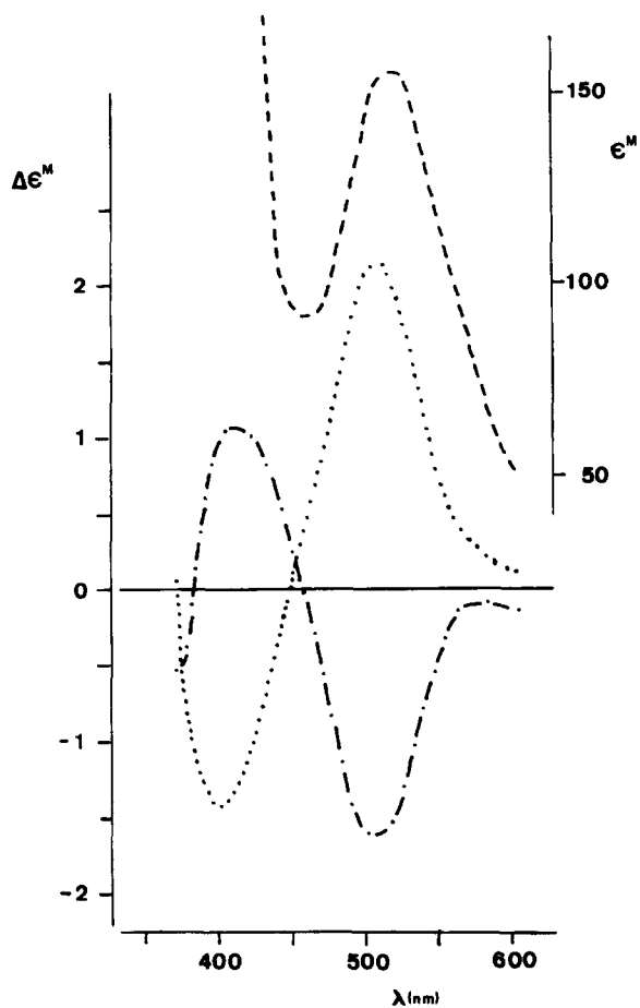
Fig. 1. Absorbance and CD spectra in the visible region. Absorbance (—), CD (···) and (— · — ·) of the \Lambda - and \Delta -complexes of \text{Co(III)(phen)}_2 with D-fructopyranose, respectively.
